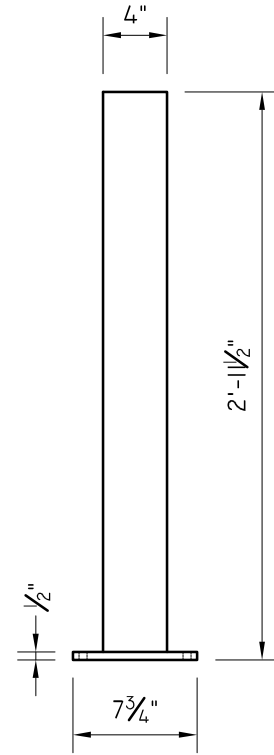
FRONT VIEW
