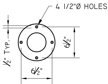
BOLT PATTERN
